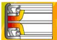
Dual Opposed Custom Metal Cased Oil Seal
